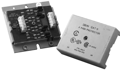
AX100826 Cat-5e, 4-pair Protector
